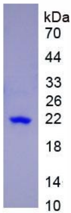
Figure 4. SDS-PAGE
