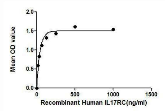
Figure 1. The binding activity of IL17RC with IL17RA.
