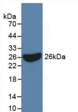
Figure 3. Western Blot
