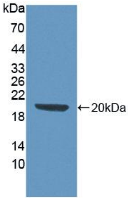
Figure 4. SDS-PAGE
