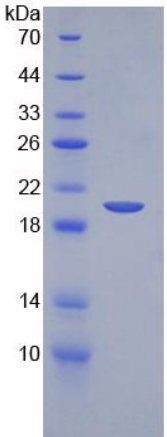
Figure 4. SDS-PAGE
