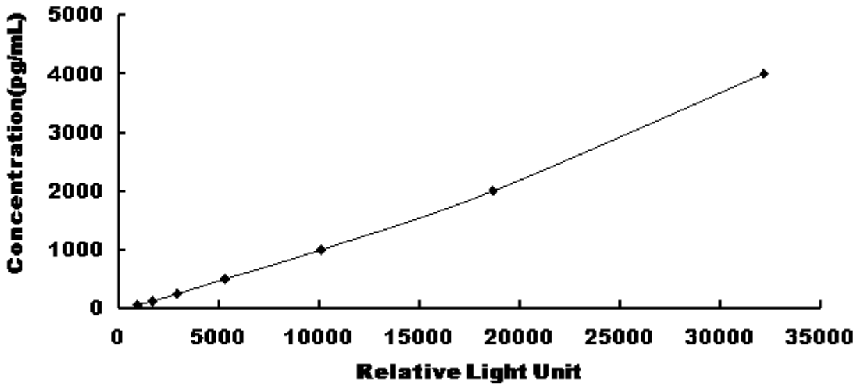
Typical Standard Curve for Equine ECF CLIA.
