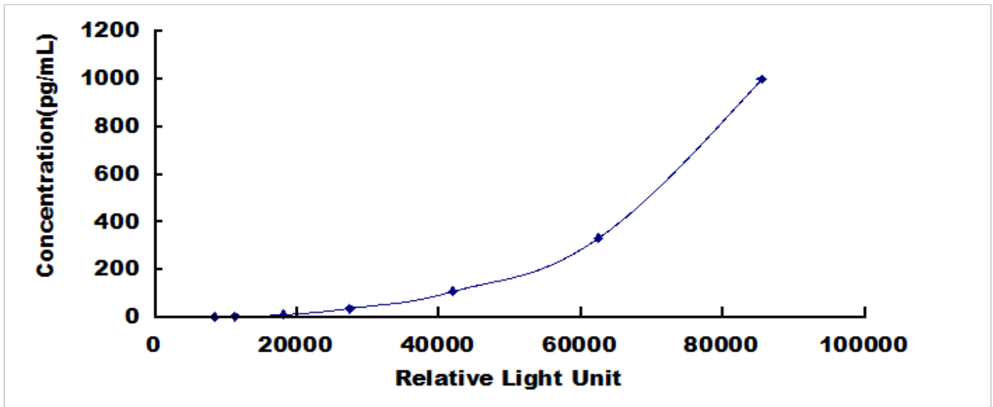
Typical Standard Curve for IL8, Human CLIA.
