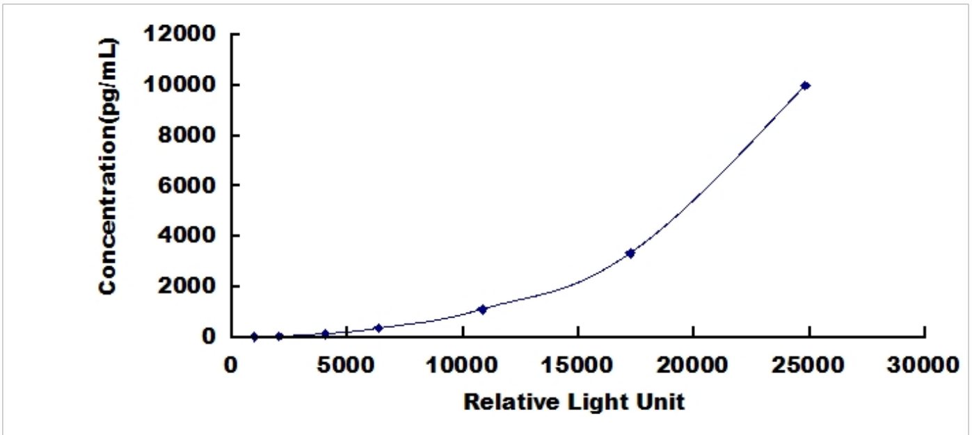
Typical Standard Curve for MIF, Mouse CLIA.
