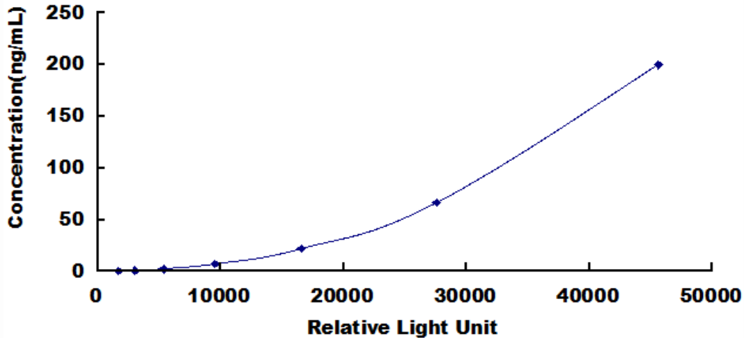
Typical Standard Curve for Myoglobin, Porcine CLIA.
