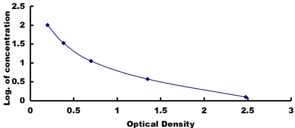
Typical Standard Curve of ELISA Assay for Arg.
