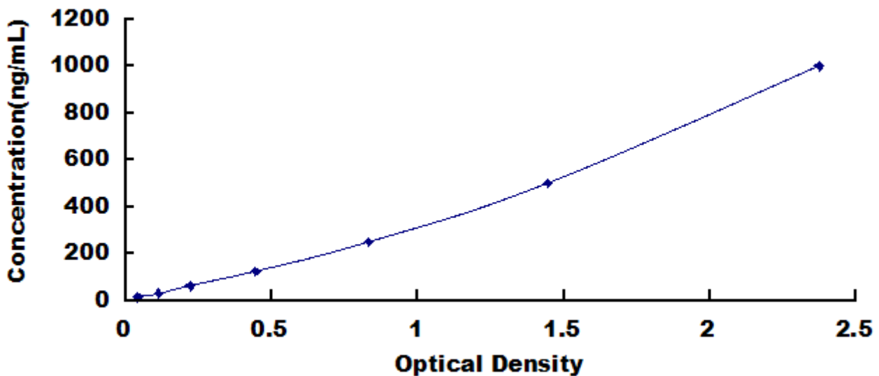
Typical Standard Curve for CDH5, Rat ELISA.
