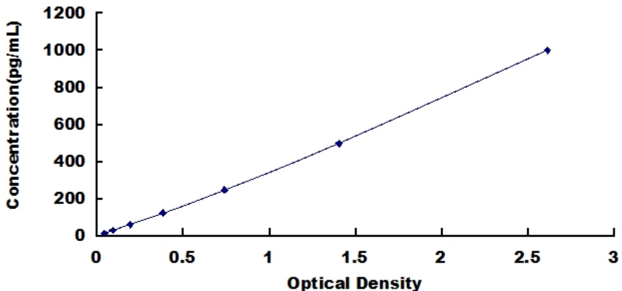
Typical Standard Curve for BRAK, Rat ELISA.
