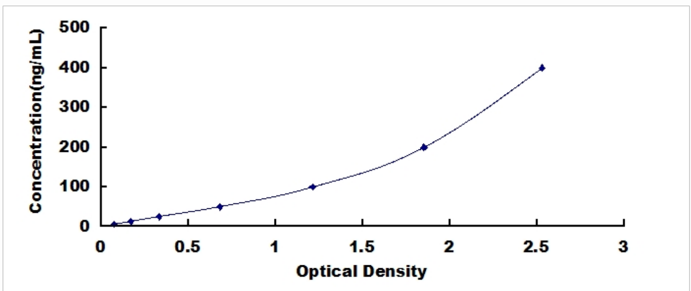
Typical Standard Curve for Clusterin, Rat ELISA.
