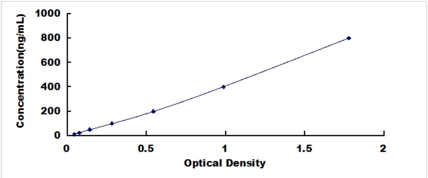
Typical Standard Curve for C5, Mouse ELISA.
