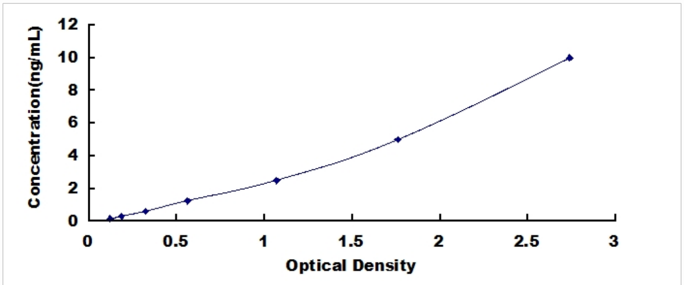
Typical Standard Curve for CYP1A1, Human ELISA.
