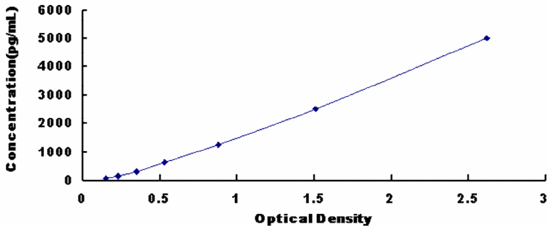
Typical Standard Curve for EMILIN2, Mouse ELISA.
