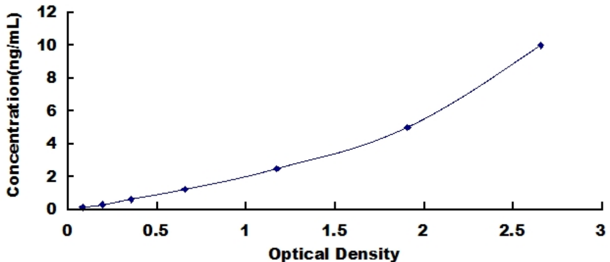
Typical Standard Curve for NR3C1, Human ELISA.
