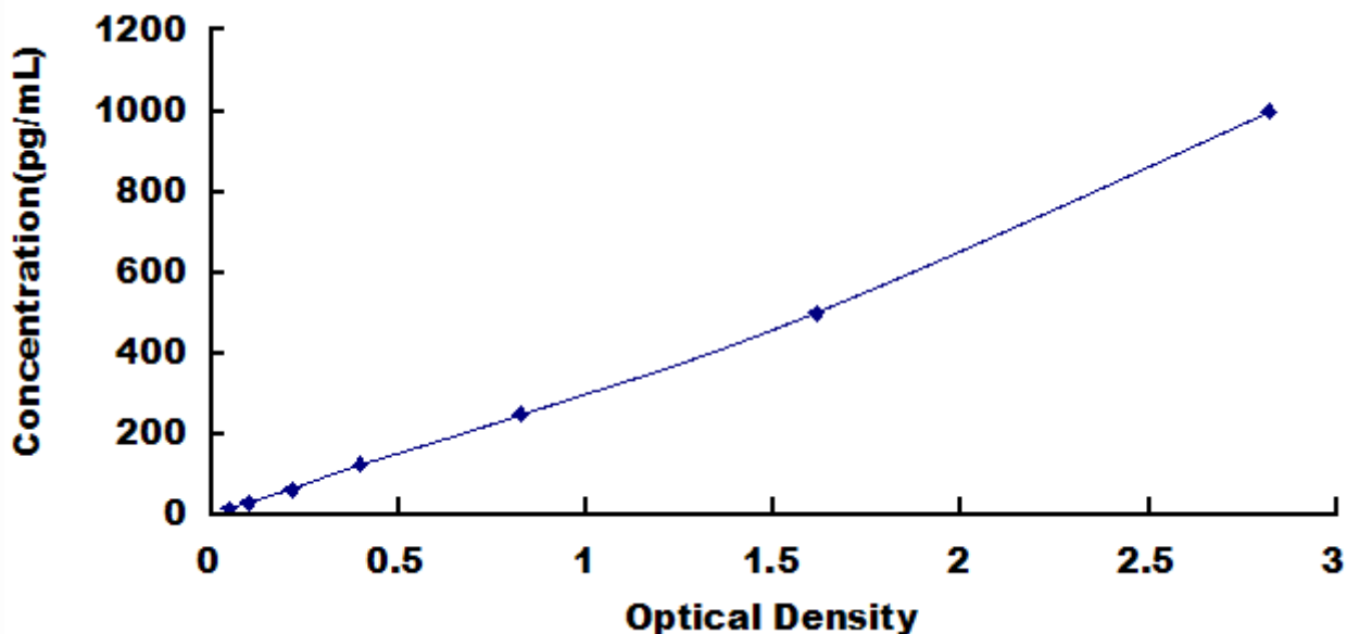
Typical Standard Curve for IL16, Mouse ELISA.
