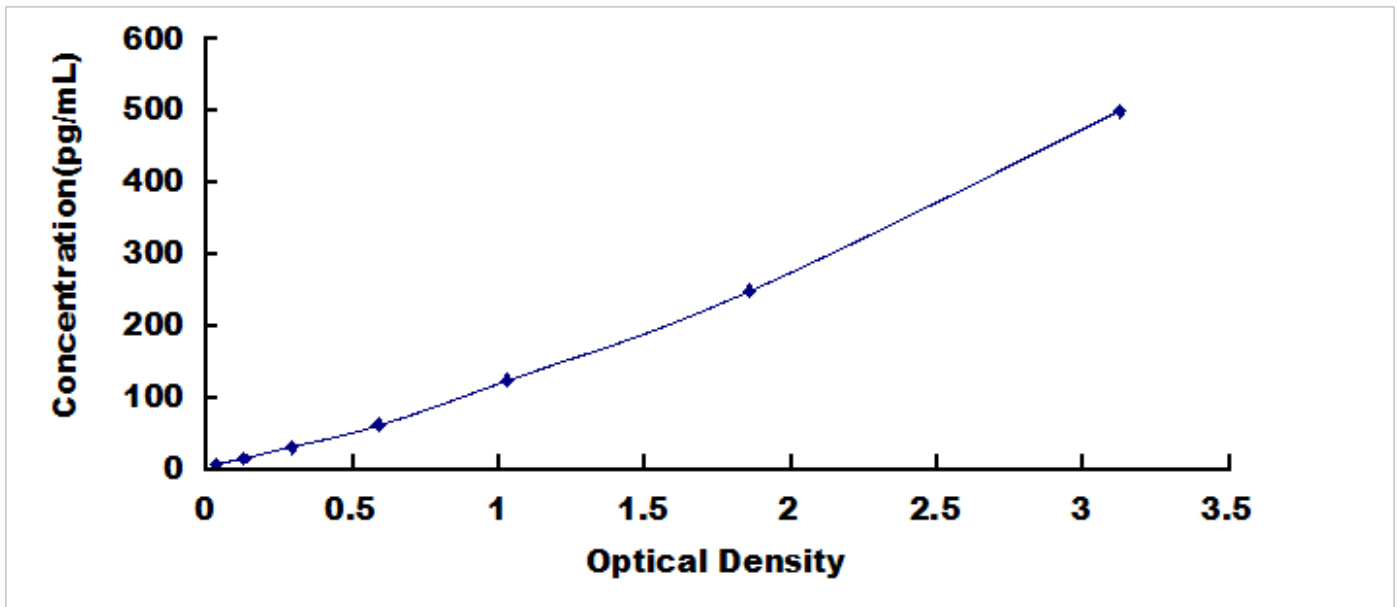
Typical Standard Curve for IL35, Mouse ELISA.
