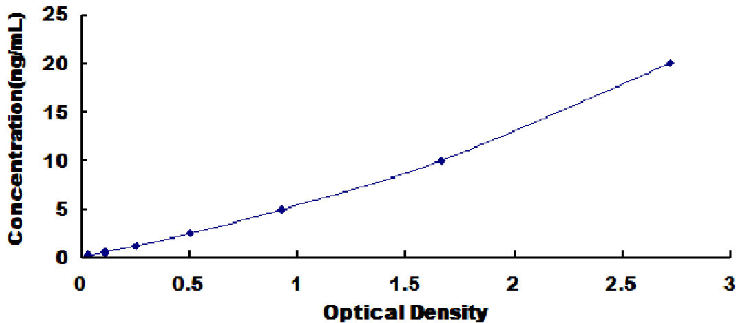
Typical Standard Curve for NOTCH2NL, Human ELISA.
