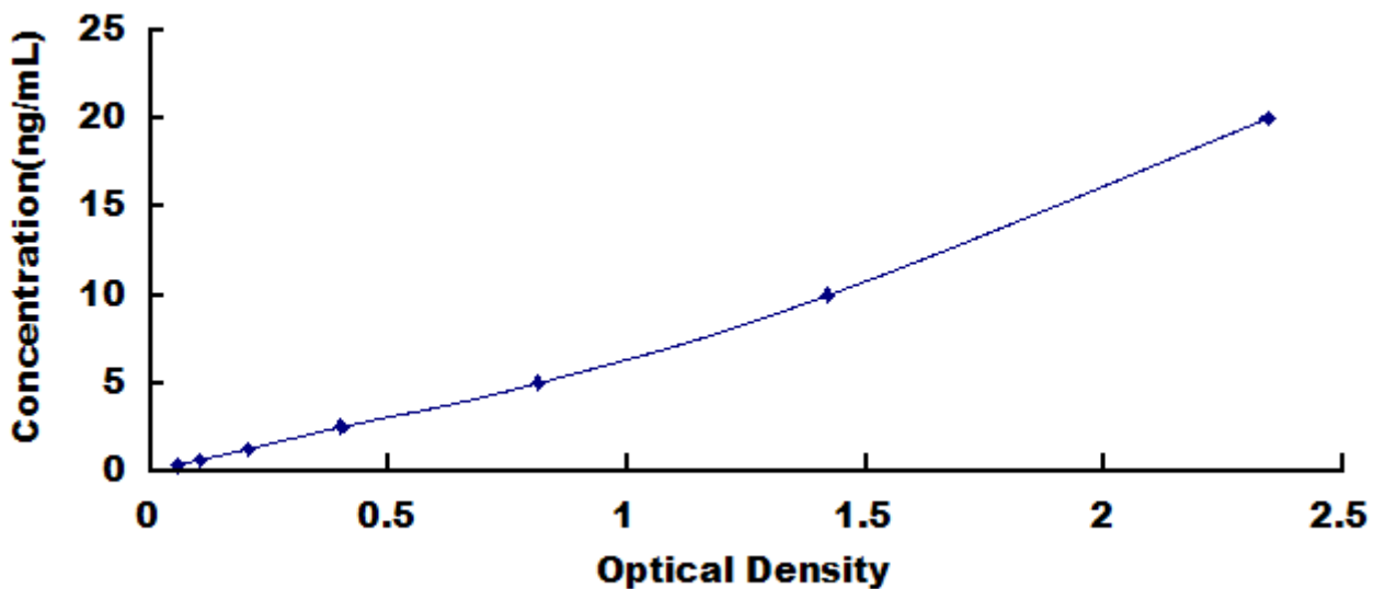
Typical Standard Curve for PDGFBB, Human ELISA.
