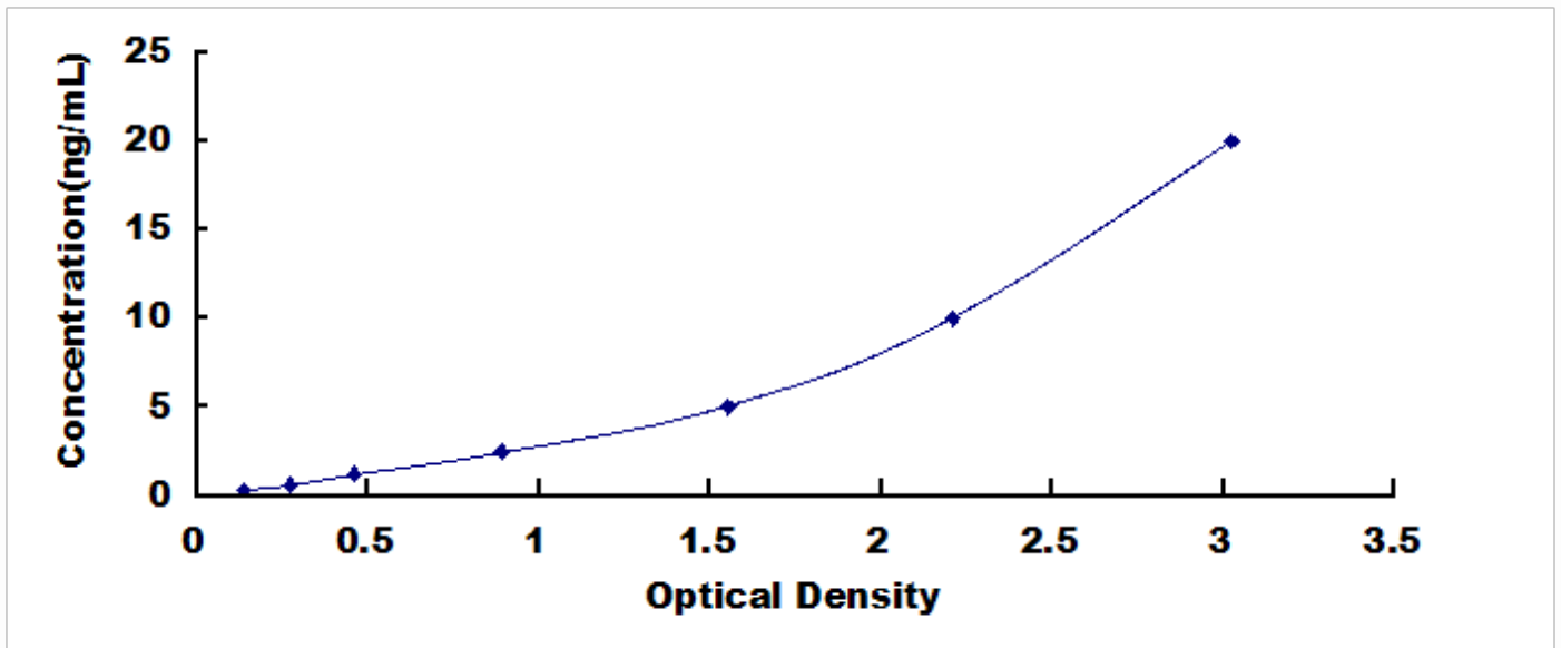
Typical Standard Curve for TLR1, Mouse ELISA.
