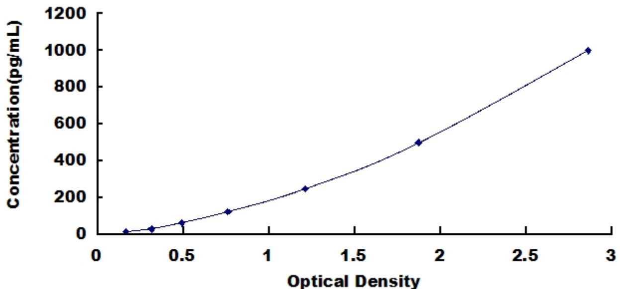
Typical Standard Curve for TREM1, Mouse ELISA.
