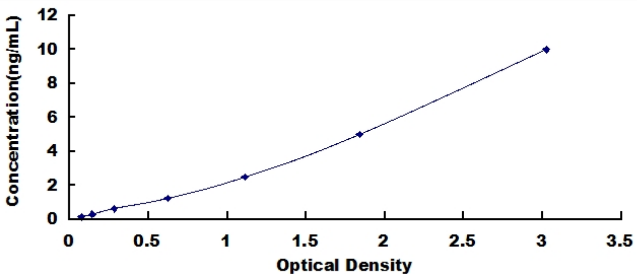
Typical Standard Curve for Trypsin, Human ELISA.
