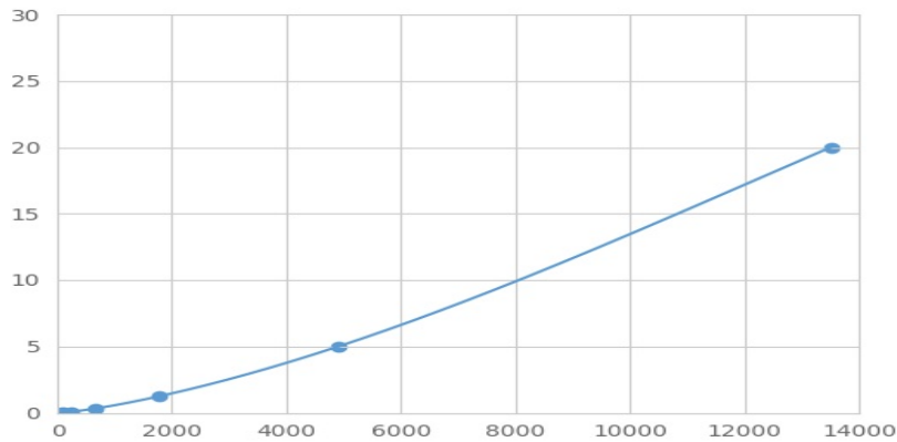
Typical Standard Curve for ABCA7 Magnetic Luminex Assay.
