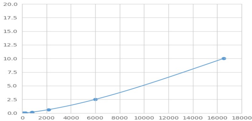
Typical Standard Curve for BHLHB3 Magnetic Luminex Assay.
