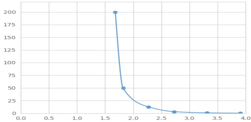
Typical Standard Curve for FGF21 Magnetic Luminex Assay.
