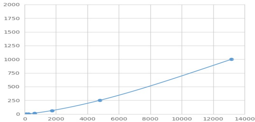
Typical Standard Curve for VEGFA Magnetic Luminex Assay.
