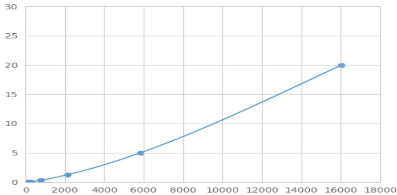
Typical Standard Curve for WNT4 Magnetic Luminex Assay.
