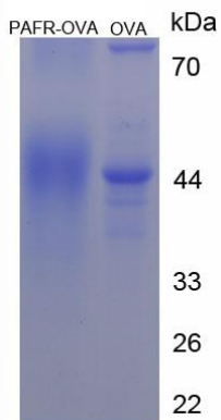
Figure 1. SDS-PAGE of OVA Conjugated PAFR
