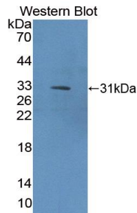
Figure. Western Blot; Sample: Recombinant COL9a1, Rat.
