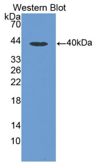
Figure. Western Blot; Sample: Recombinant MIP1a, Mouse.
