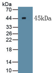
Figure. Western Blot; Sample: Recombinant MyoD, Human.
