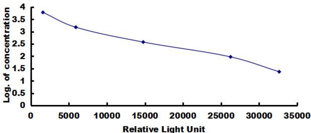
Typical Standard Curve for 8-OHdG CLIA.
