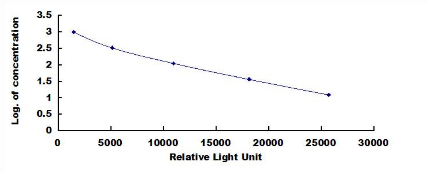
Typical Standard Curve for Estradiol CLIA.
