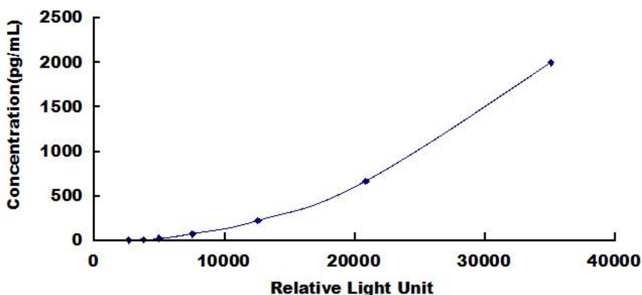
Typical Standard Curve for TSLP, Human CLIA.
