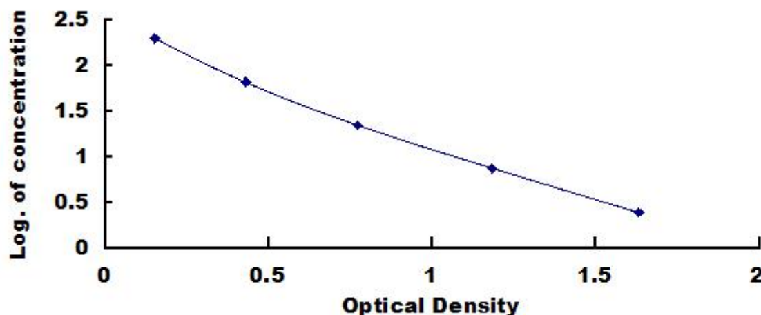
Typical Standard Curve for 7-DHC ELISA.
