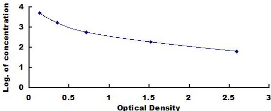
Typical Standard Curve for Acetylcarnitine ELISA.
