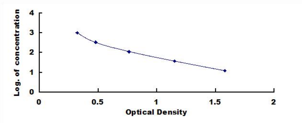
Typical Standard Curve for Adrenomedullin, Human ELISA.
