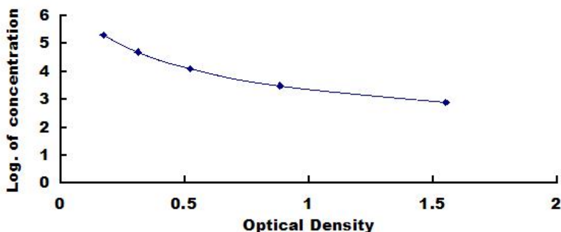
Typical Standard Curve for a1AT, Canine ELISA.
