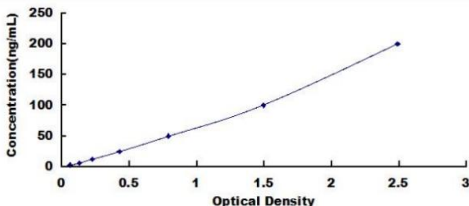
Typical Standard Curve for Anti-NPHN, Human ELISA.
