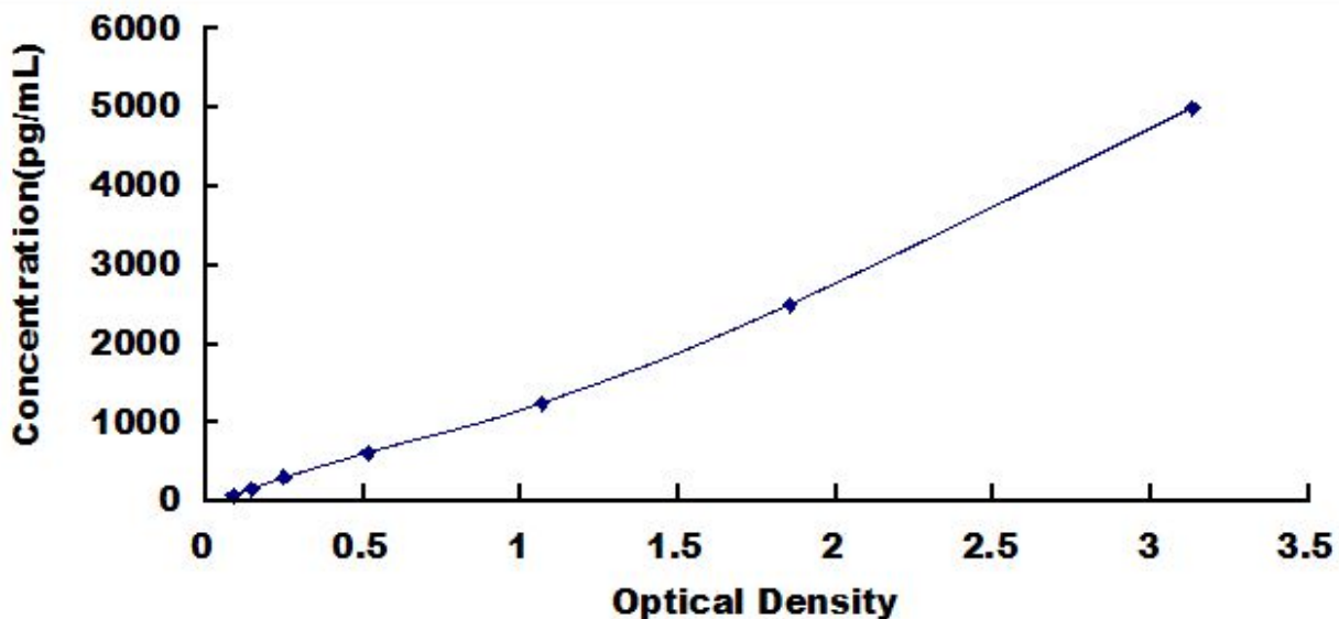
Typical Standard Curve for BAD, Human ELISA.
