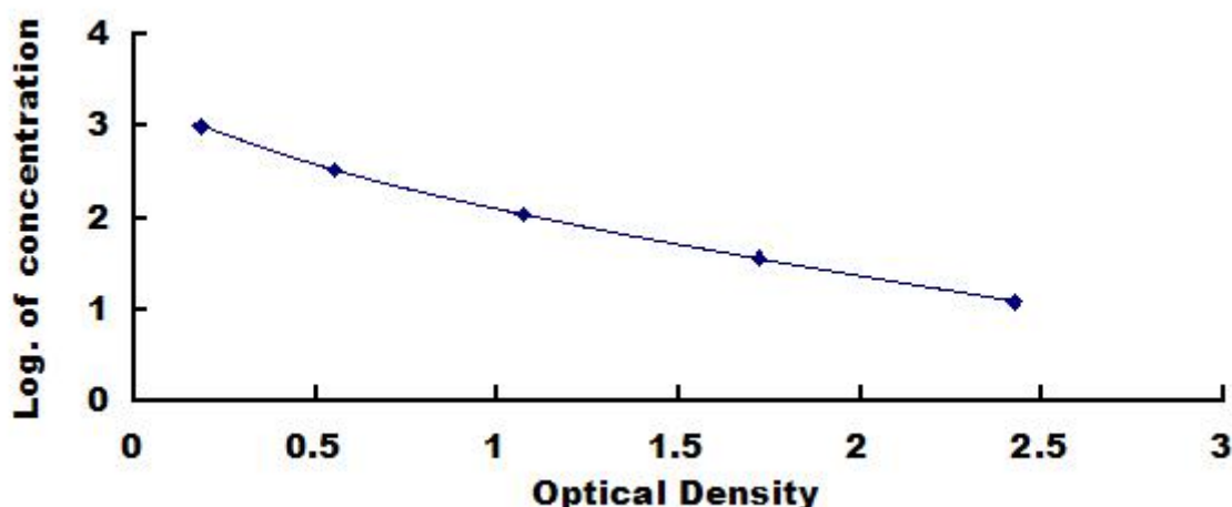
Typical Standard Curve for Calcitonin, Mouse ELISA.
