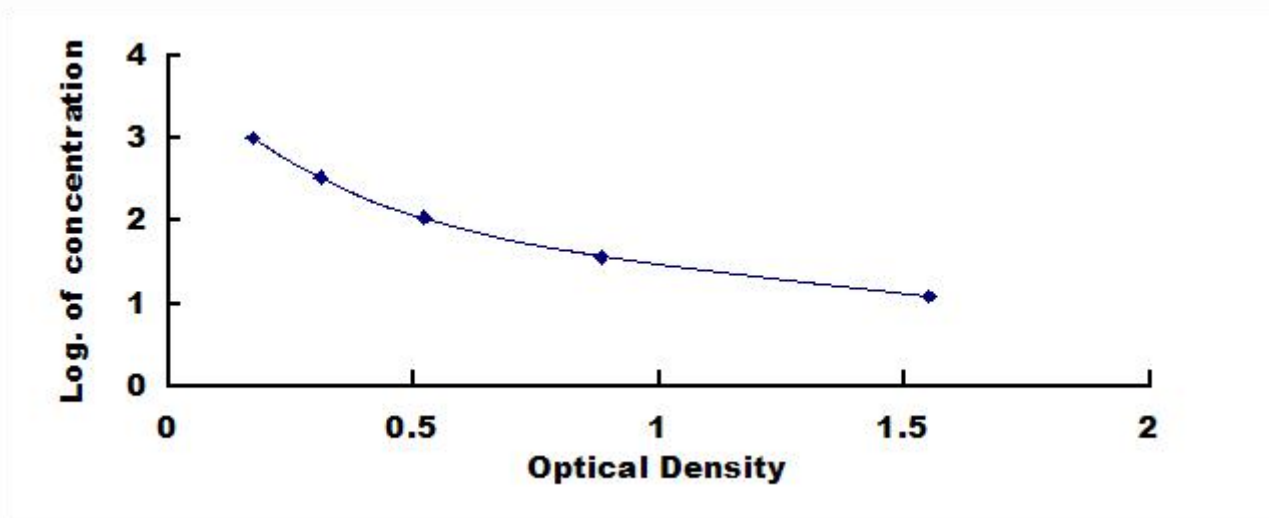
Typical Standard Curve for Calcitonin, Rat ELISA.
