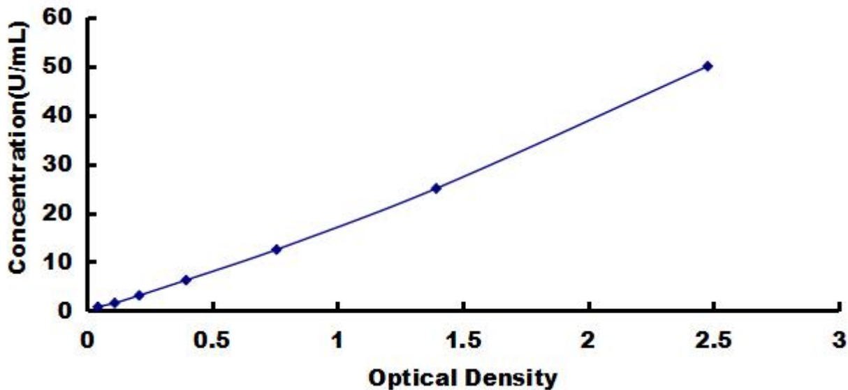
Typical Standard Curve for CA19-9, Human ELISA.
