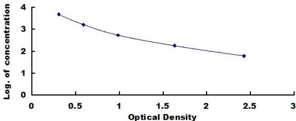
Typical Standard Curve for CML ELISA.
