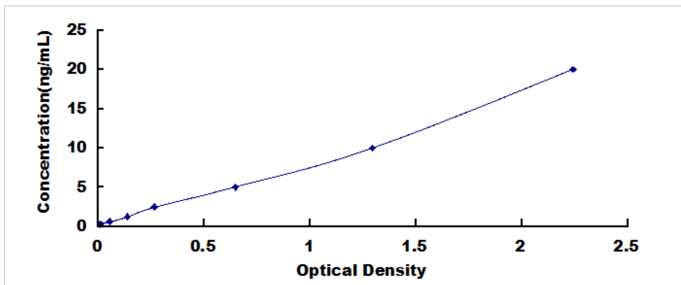
Typical Standard Curve for CASP1, Human ELISA.
