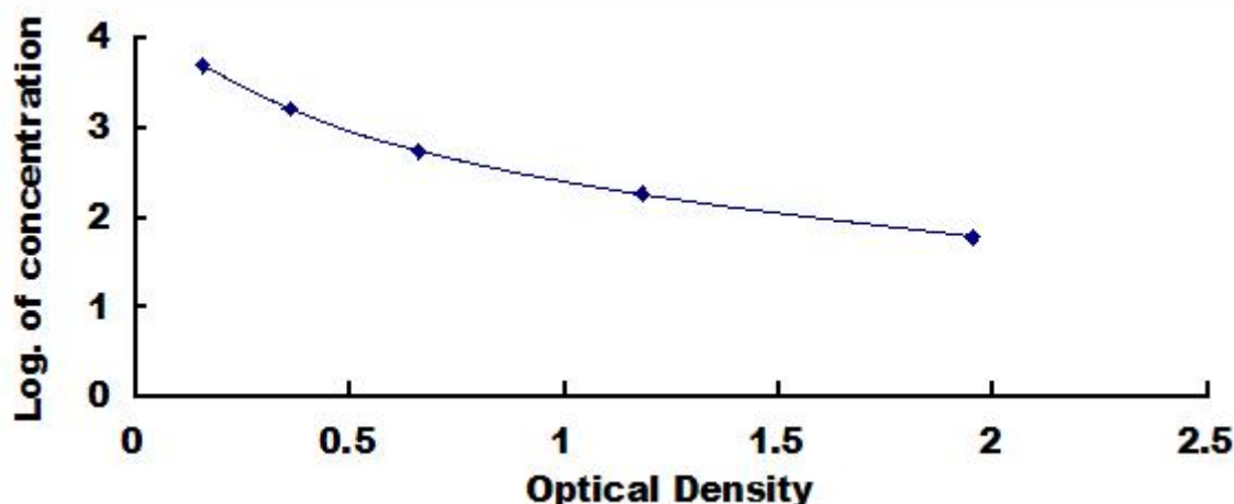
Typical Standard Curve for Cholic Acid ELISA.
