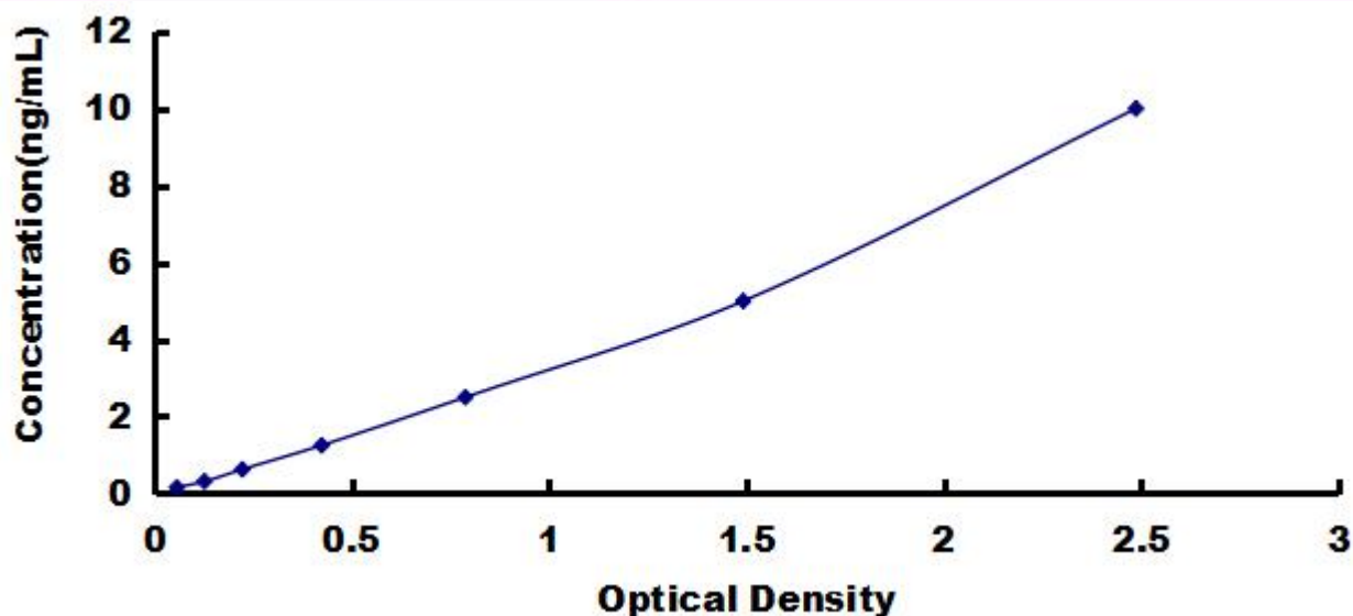
Typical Standard Curve for CLDN2, Mouse ELISA.
