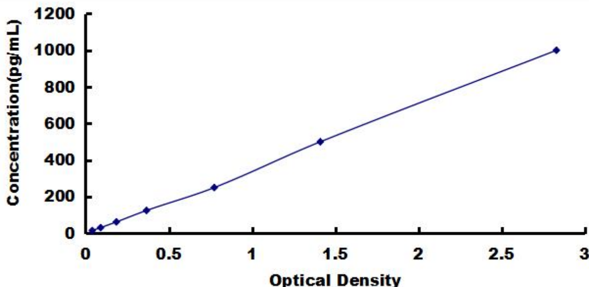
Typical Standard Curve for MCSF, Rat ELISA.
