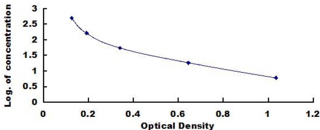
Typical Standard Curve for Corticosterone ELISA.
