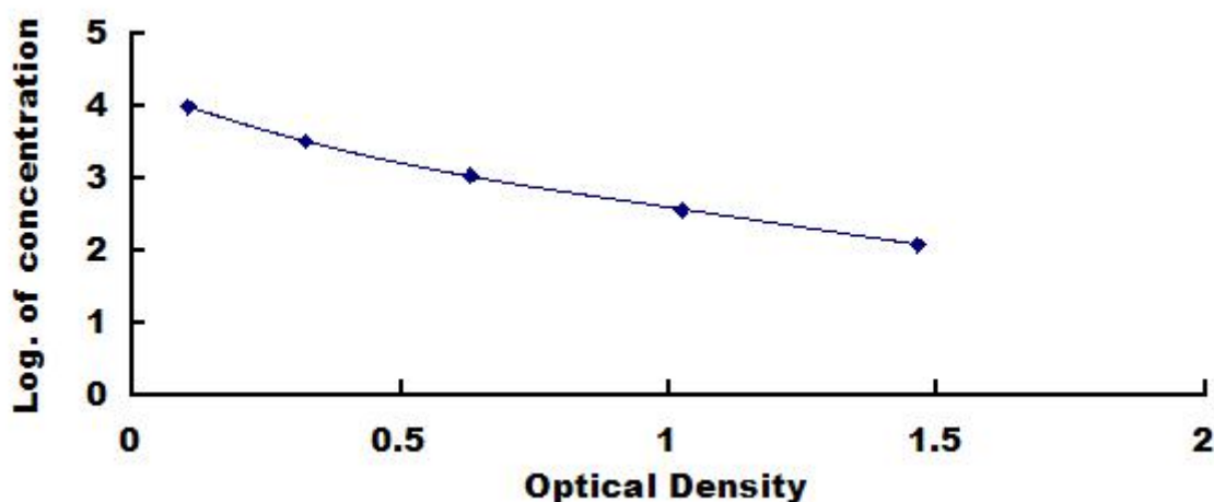
Typical Standard Curve for CTXII, Human ELISA.
